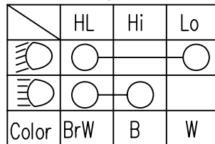
Switch, high/low beam
